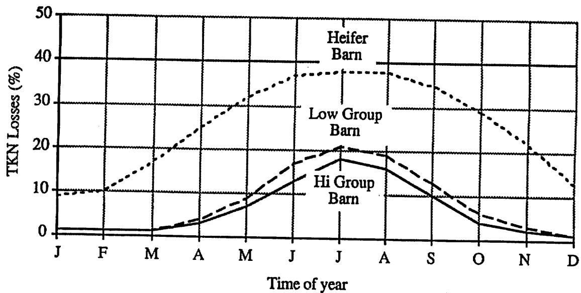
Figure 3. Ammonia volatilization losses for Farm B animal housing facilities as a function of time of year.
