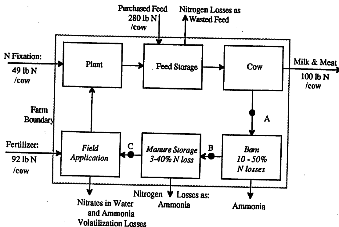
Figure 1. Illustration of nitrogen flows for dairy farm and the points at which this activity tried to measure nitrogen concentration (A, B, and C).
