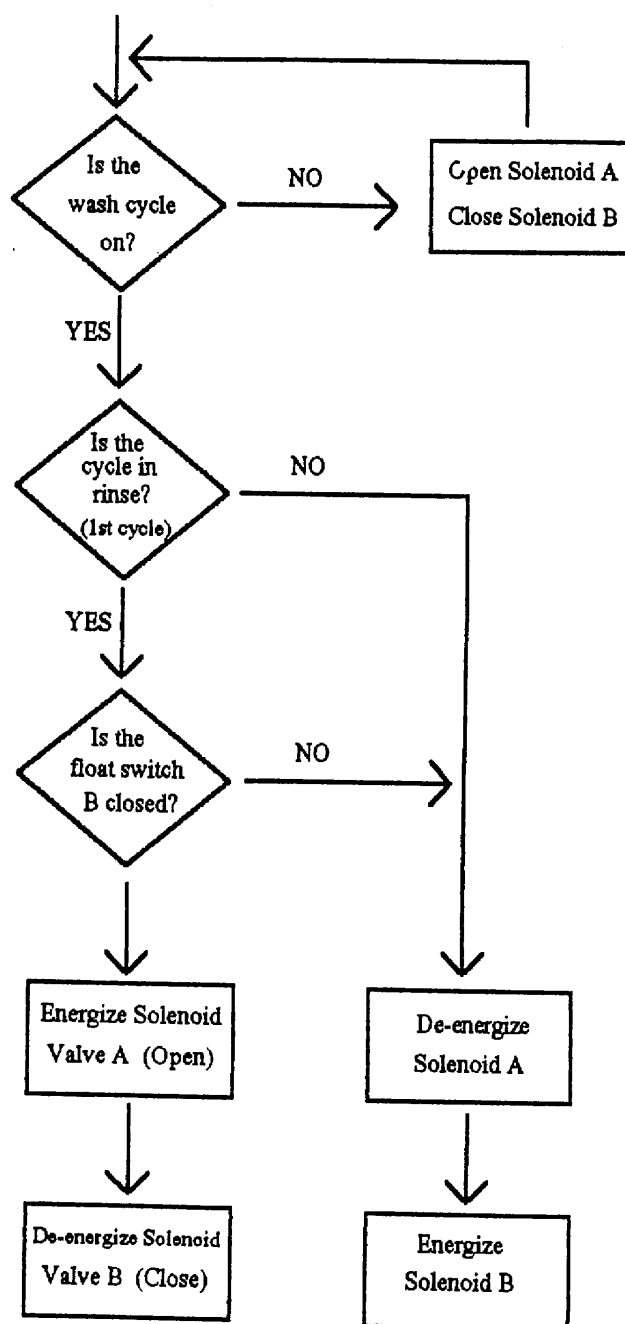
Figure 15. Milk center washwater control logic
