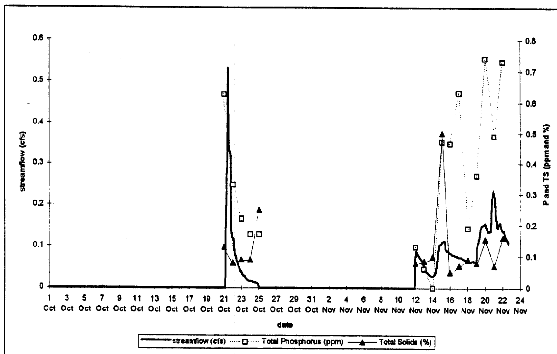
Fig. 6: Streamflow in cubic feet per second (cfs), Total Phosphorus (ppm), and Total Solids (%) concentration in streamflow from Farm A drainage basin 10/1/95 - 11/22/95
