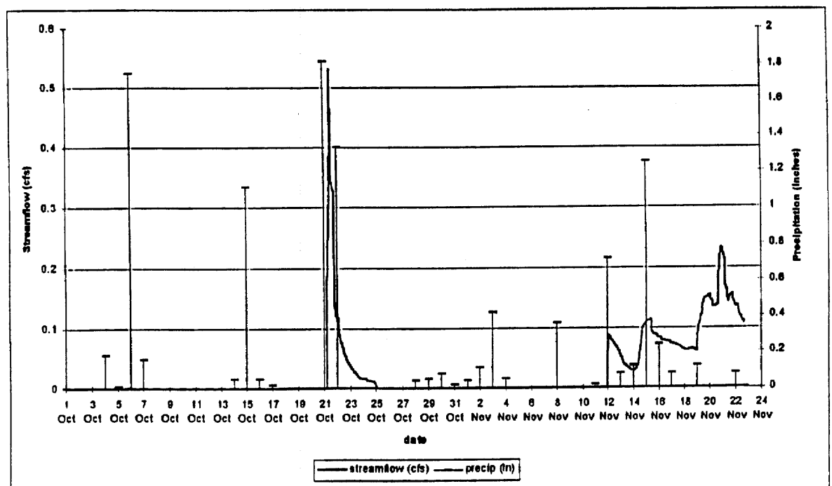
Fig. 2: Measured streamflow in cubic feet per second (cfs) from the Farm A drainage basin, and precipitation as recorded at the Aurora Farm Research Station 10/1/95 - 11/22/95
