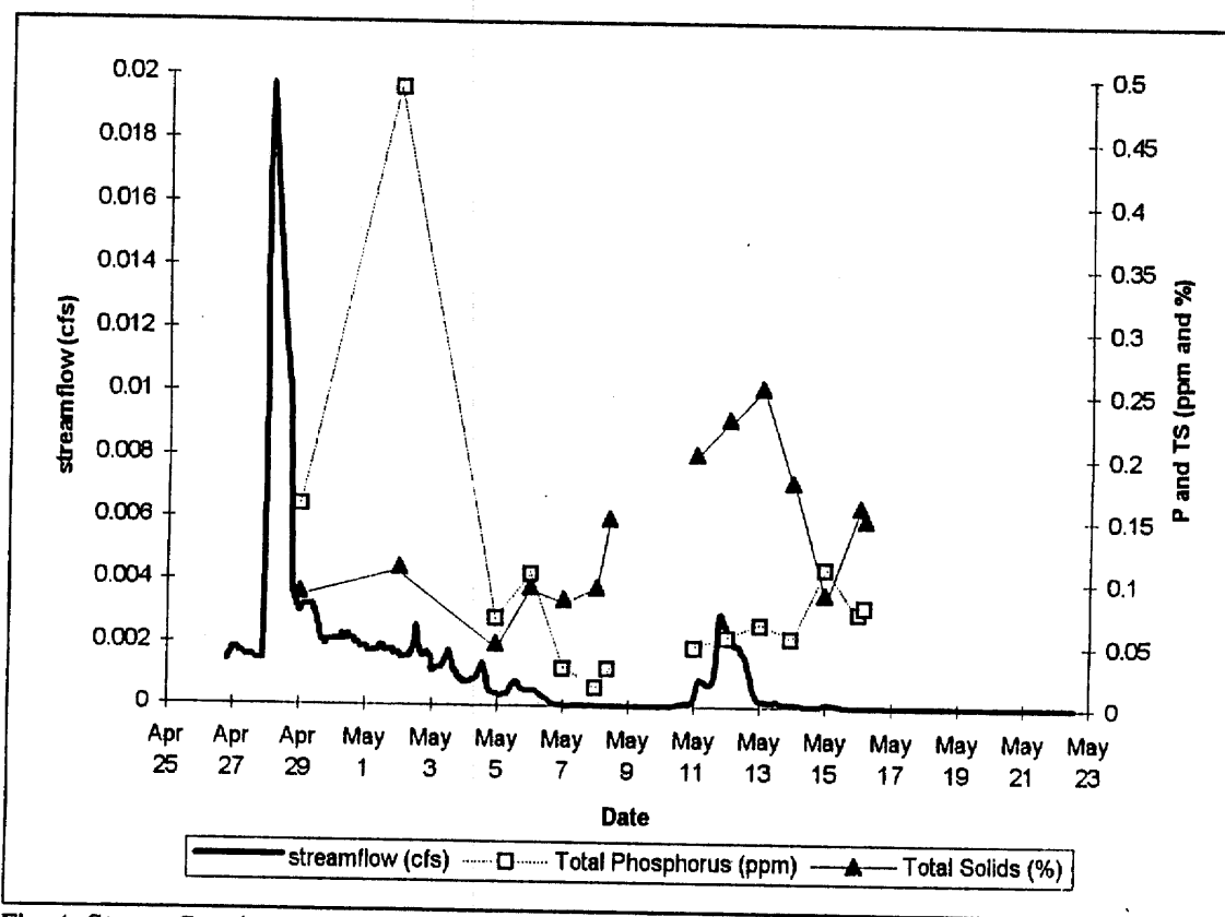
Fig. 4: Streamflow in cubic feet per second (cfs), Total Phosphorus (ppm), and Total Solids (%) concentration in streamflow from Farm A drainage basin 4/26/95 - 5/26/95
