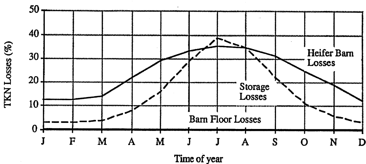
Figure 5. Ammonia volatilization losses for Farm A farm facilities as a function of time of year.
