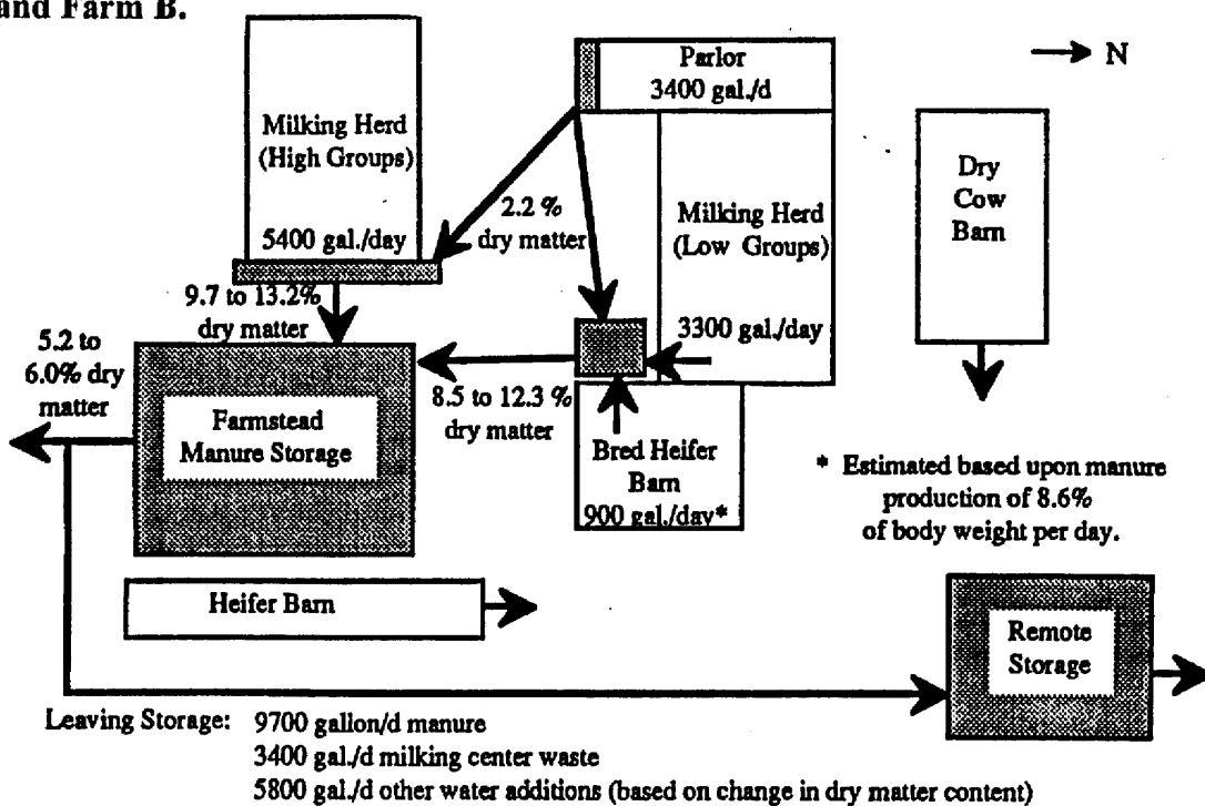
Figure 2. Dry matter characteristics and quantities of manure and waste water handled on Farm A and Farm B.
