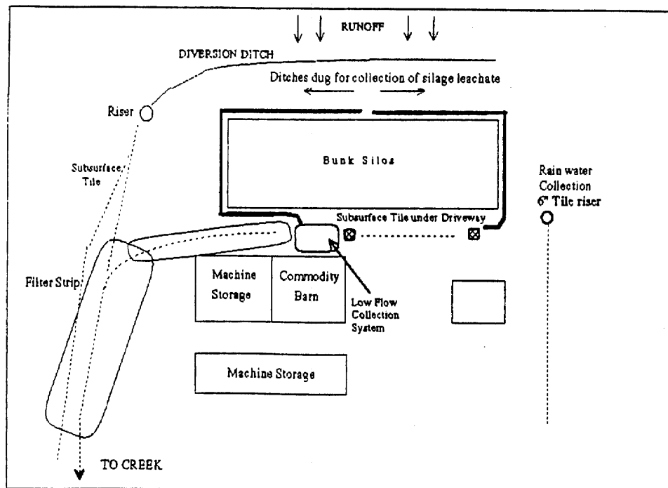
Figure 9. Overview of bunk silos
