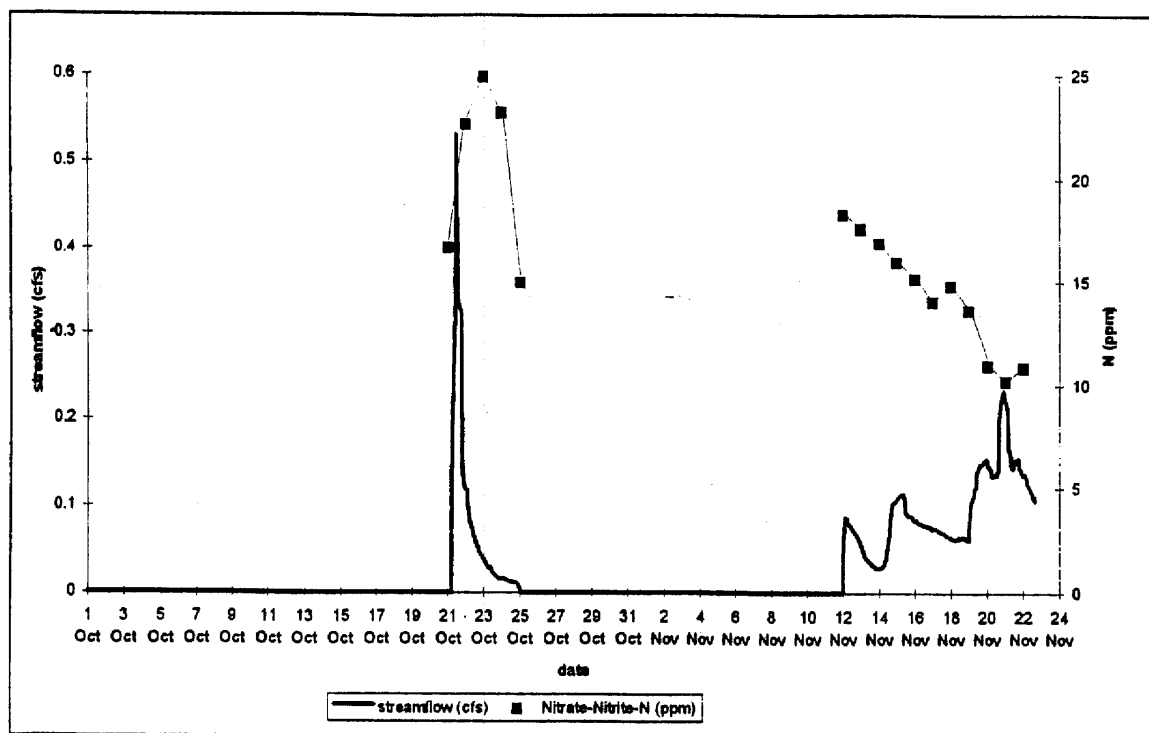
Fig. 5: Streamflow in cubic feet per second (cfs) and Nitrate-Nitrite-N concentration (ppm) in streamflow from Farm A drainage basin 10/1/95 - 11/22/95
